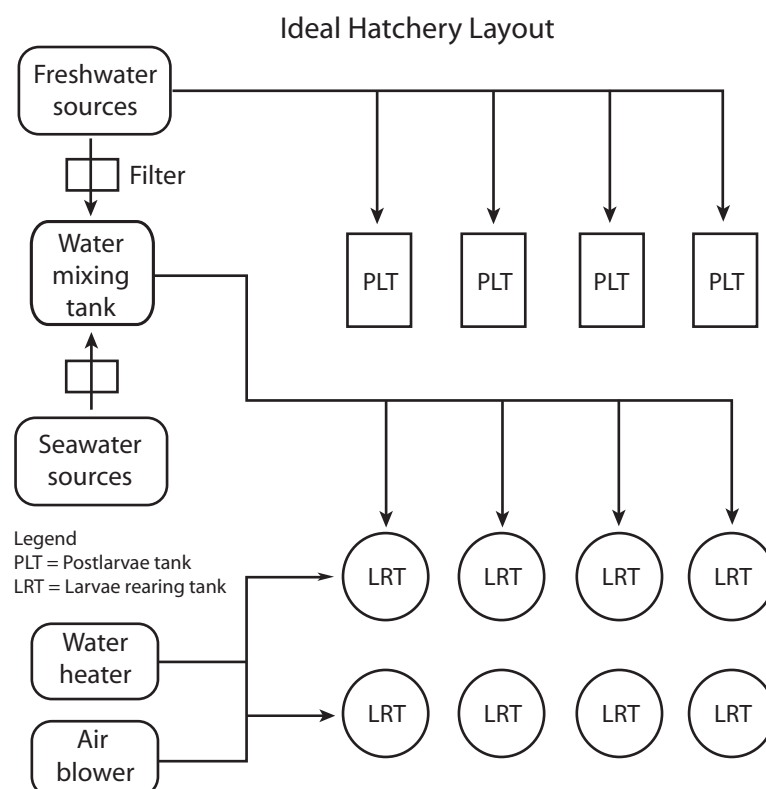
Fig. 5. Ideal layout of a semi-commercial/back-yard freshwater prawn hatchery
