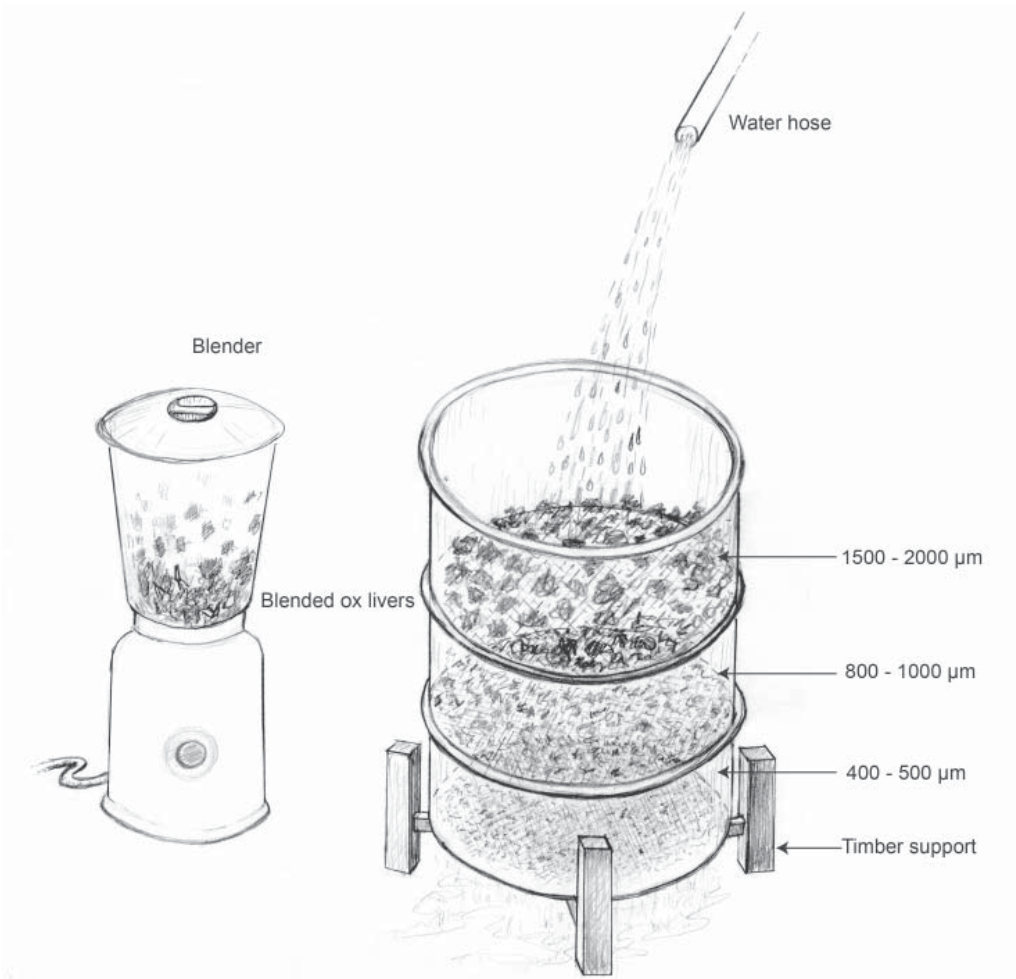
Fig. 10. Preparation of ox liver
